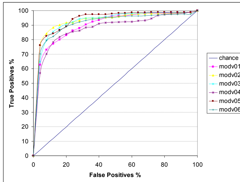
Figure 2: ROC curves for the different versions of the model
