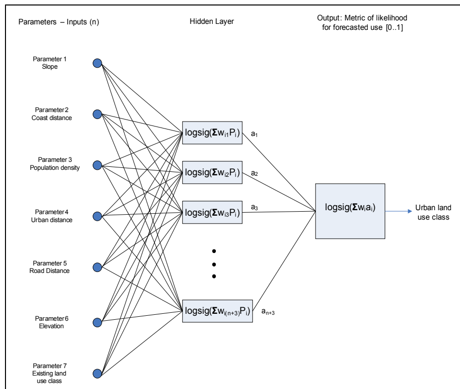
Figure 1: Conceptual diagram of the initial neural-network model
