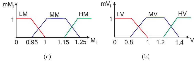
Fig. 1. From numerical features to belief. (a) Mean value. LM (function f_1 , red color), MM (function f_2 , blue color) and HM (function f_3 , green color) functions correspond to low, medium and high values of the normalized mean of image intensity, respectively. (b) Variance. LV (function g_1 , red color), MV (function g_2 , blue color) and HV (function g_3 , green color) correspond to low, medium and high values of the normalized variance of image intensity, respectively.
